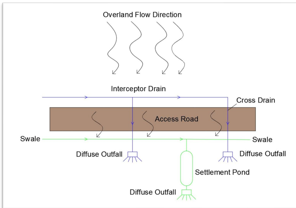
Plate 2-4: Drainage Diagram
